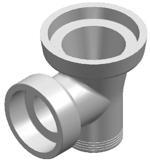
ISOMETRIC VIEW 1:5
