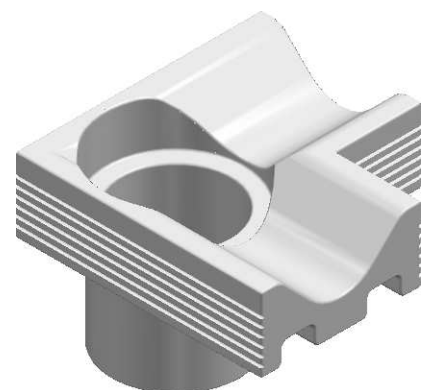
ISOMETRIC VIEW 1:5
