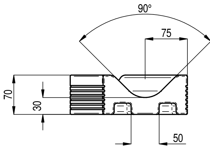
VIEW A
