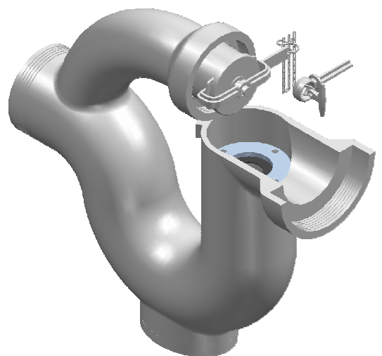
ISOMETRIC VIEW 1:10
