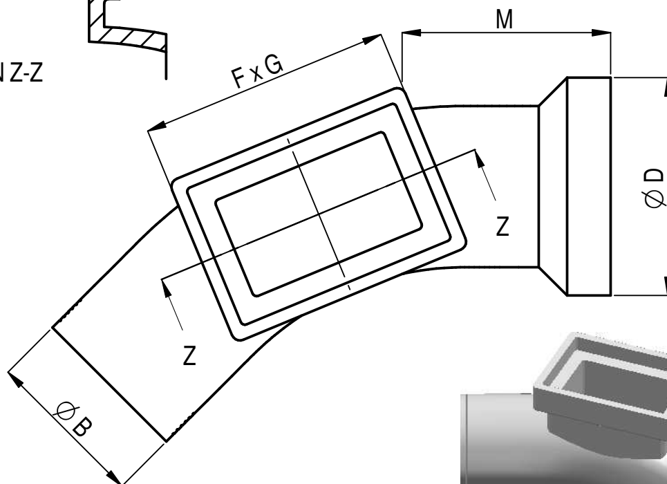
ISOMETRIC VIEW 1:10
