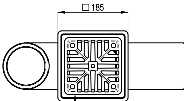
CAST IRON SQUARE GRATE
